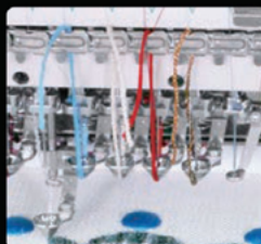
Multi cording Device Embroidering 6 various types/colors of cords
